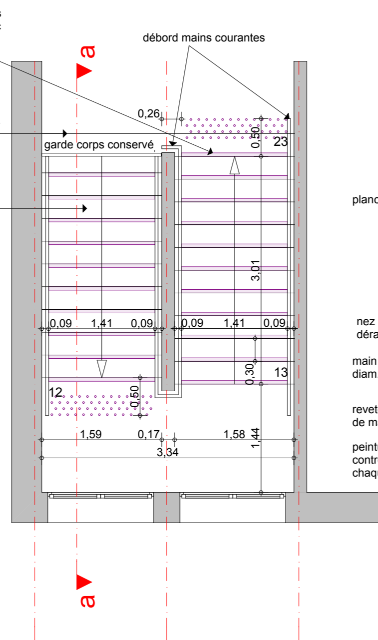
plan R+1
